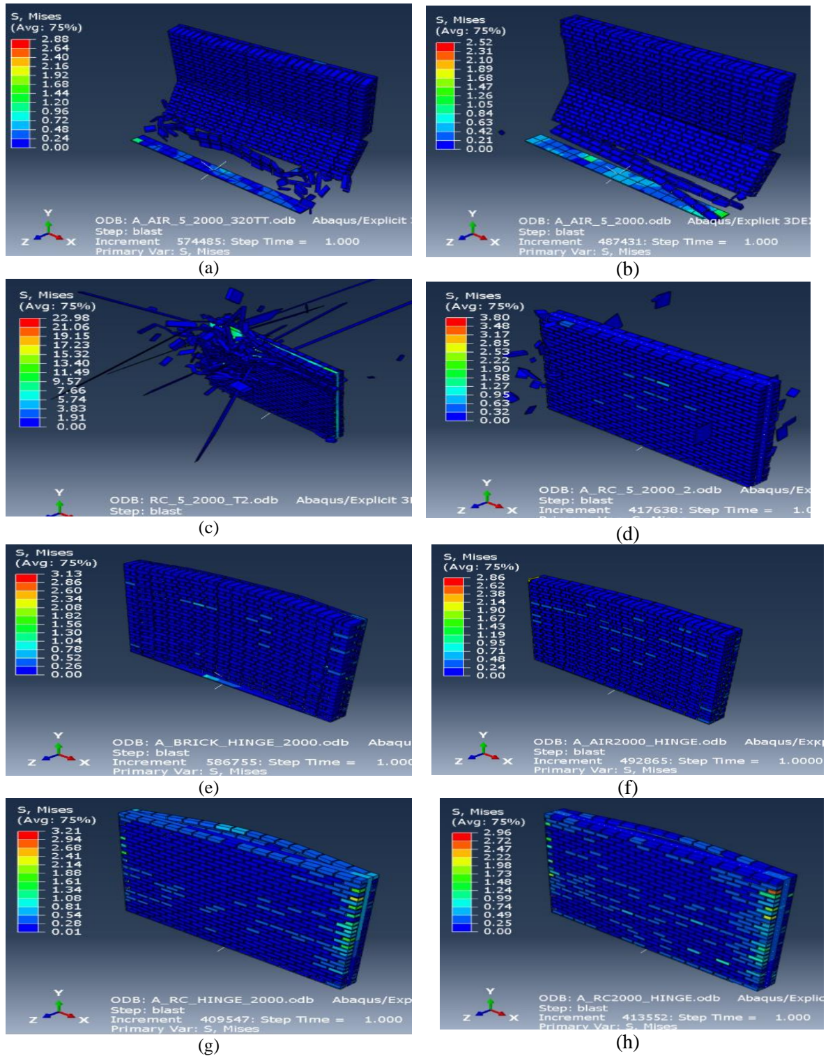
Figure (5): Distribution of Von mises stress (MPa): (a) M1; (b) M2; (c) M3; (d) M4; (e) M5; (f) M6; (g) M7; (h) M8.
