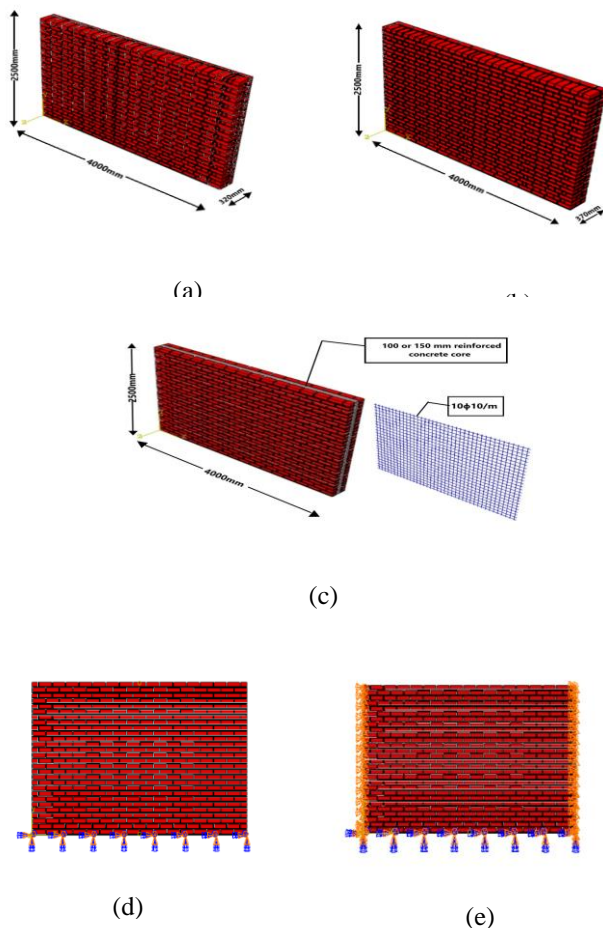
Figure (2): Finite element models: (a), (b) Brick models; (c) RC core model; (d), (e) Boundary conditions of the walls (fixed bottom -fixed bottom with hinge sides).
