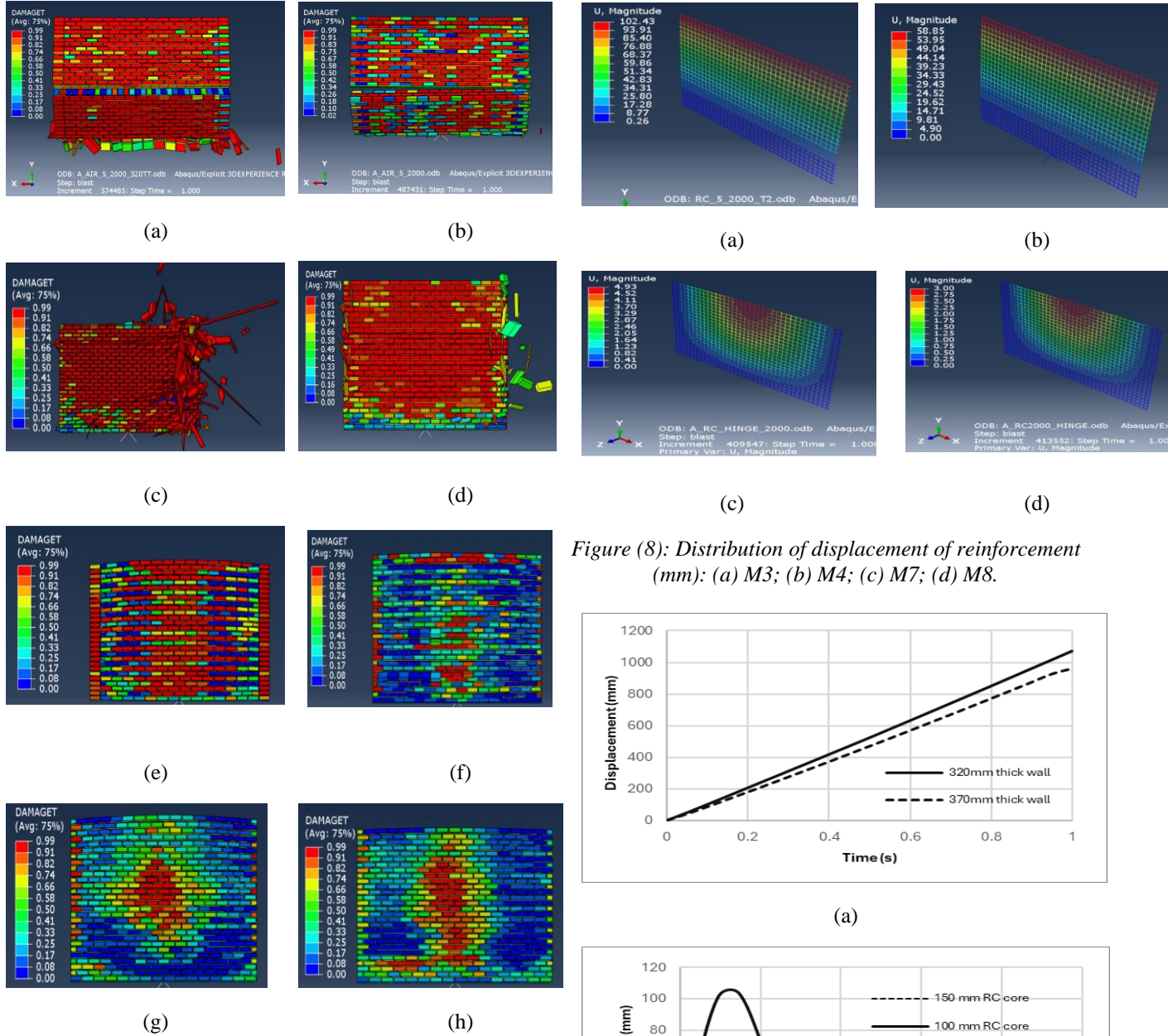
Figure (7): Damage pattern across rear side of walls: (a) M1; (b) M2; (c) M3; (d) M4; (e) M5; (f) M6; (g) M7; (h) M8.
