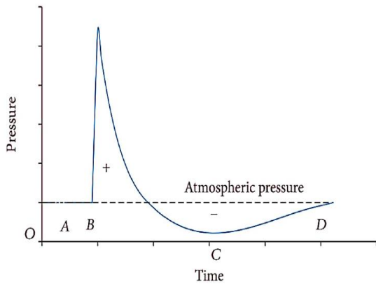
Figure (1): Pressure time history for free explosion [7].
