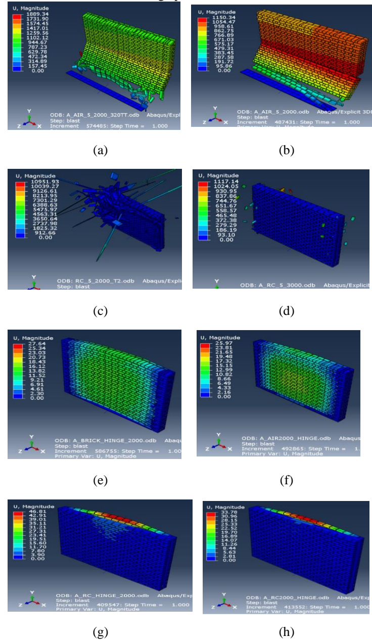
Figure (4): Displacement distribution (mm): (a) M1; (b) M2; (c) M3; (d) M4; (e) M5; (f) M6; (g) M7; (h) M8.
